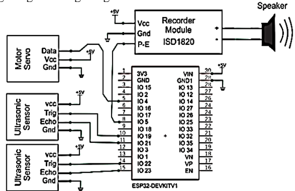
Figure 2. Hardware circuit board schematic.
